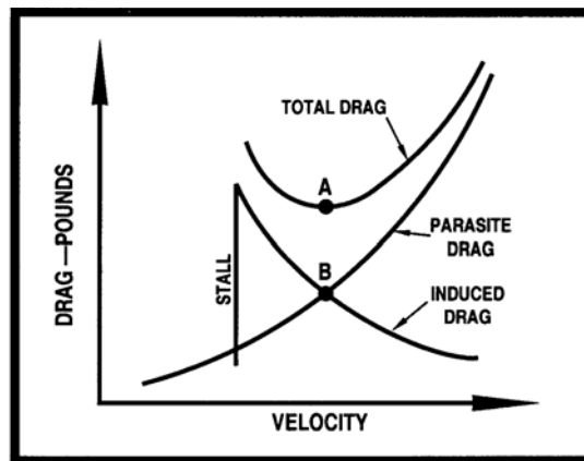
Figure 2 – Drag Chart
